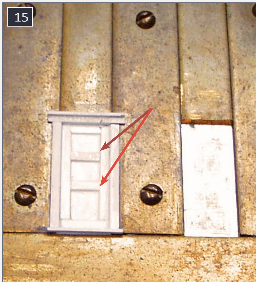
15. The rest of the door rails have been added creating the three panels needed for the door.
